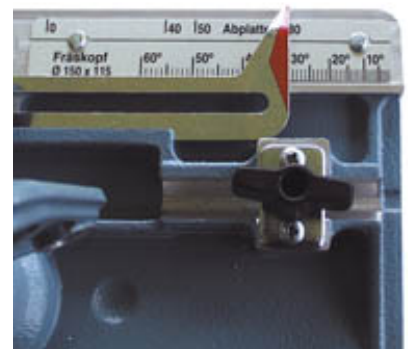
Just position the machine on the skew notch edge of reference.
